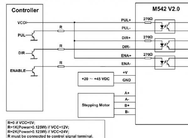
Figure 10: Typical connection
