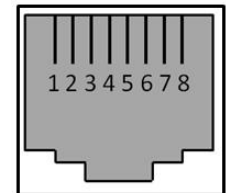
RJ45 Port
