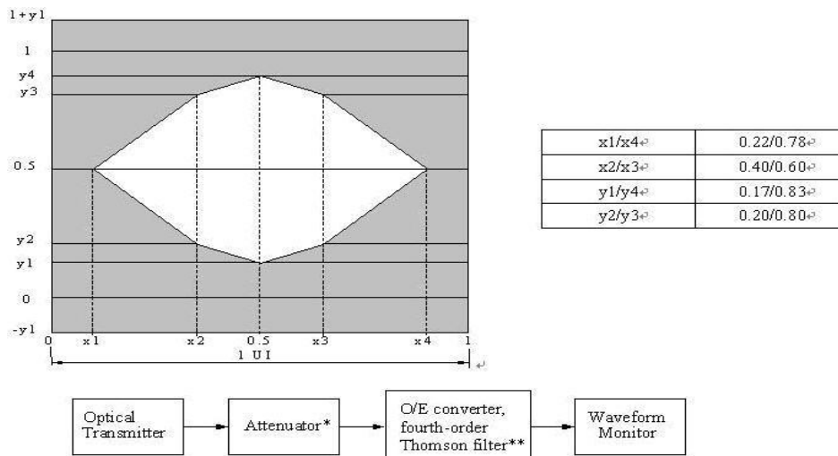
Figure 1: Transmitter Eye Mask Definitions
