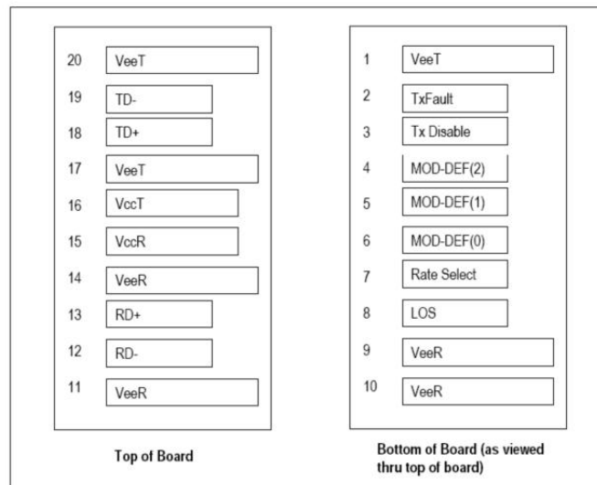
Figure 3:Pin Out Drawing (Top view)
