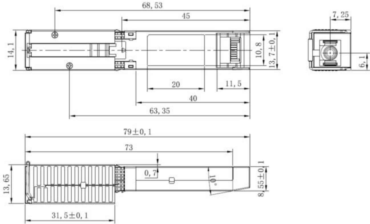
Figure 5: Package Outline (unit: mm)
