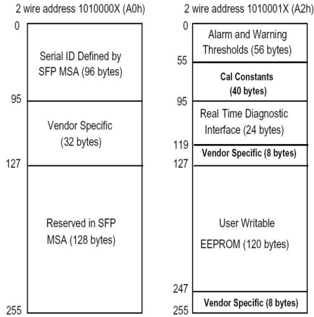
Figure 2:EEPROM Information
