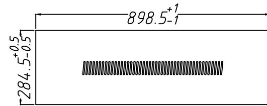
side panel
