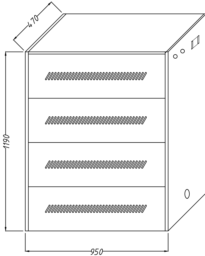
Appearance diagram
