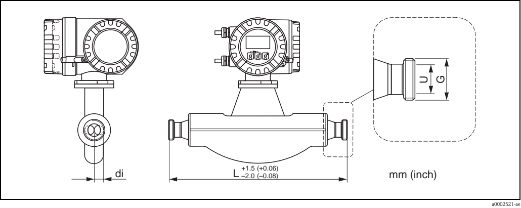
DIN 11864-1 Form A (threaded hygienic connection)
