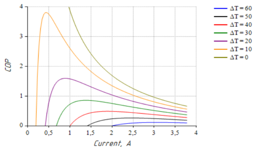
COP vs. Current (at T_{hot} = 27^{\circ}C )
