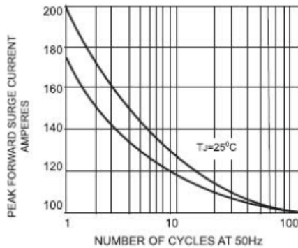
FIG.1 - MAXIMUM FORWARD SURGE CURRENT
