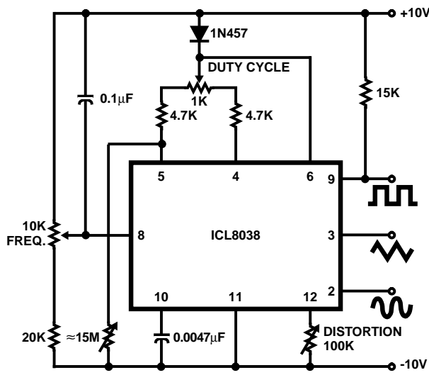
FIGURE 8. VARIABLE AUDIO OSCILLATOR, 20Hz TO 20kHz
