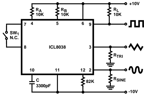
FIGURE 1. TEST CIRCUIT
