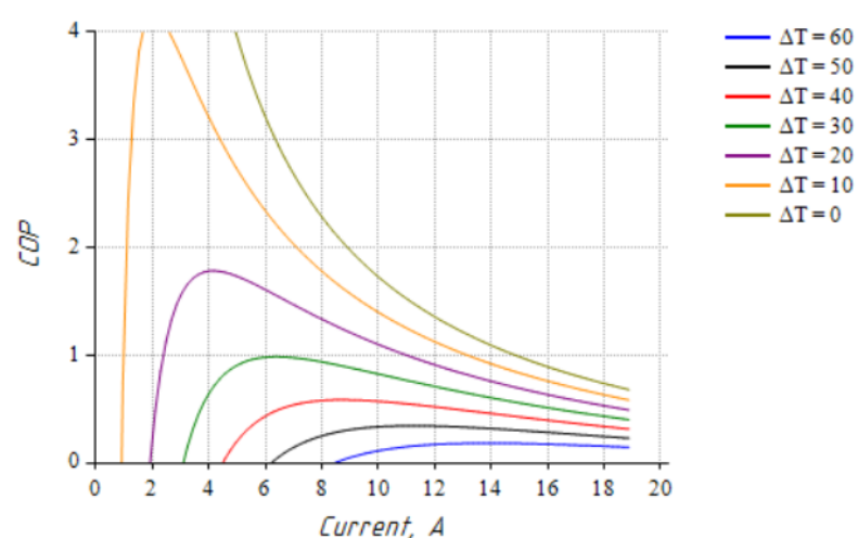
COP vs. Current (at T_{hot} = 50^{\circ}\text{C} )
