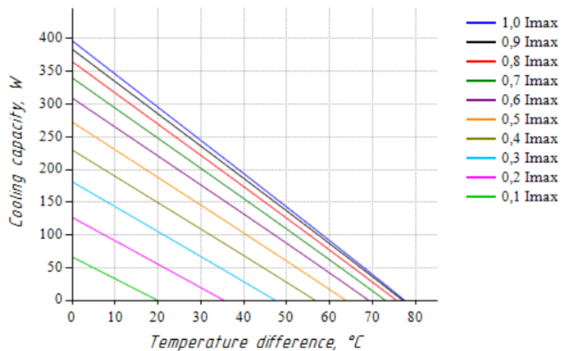
Cooling capacity vs. Temperature difference (at T_{hot} = 50^{\circ}\text{C} )
