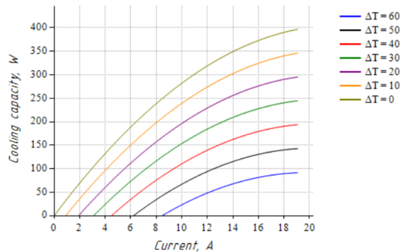
Cooling capacity vs. Current (at T_{hot} = 50^{\circ}\text{C} )
