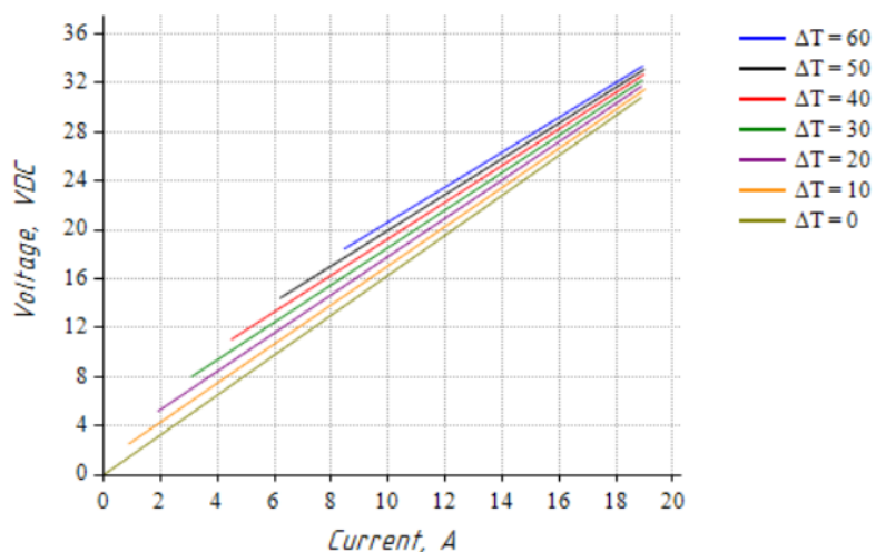
Voltage vs. Current (at T_{hot} = 50^{\circ}\text{C} )
