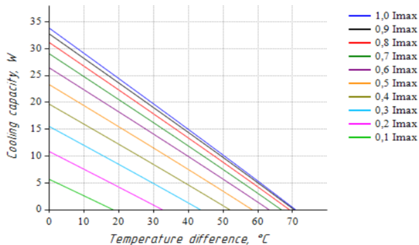
Cooling capacity vs. Temperature difference (at T_{hot} = 27^{\circ}C )
