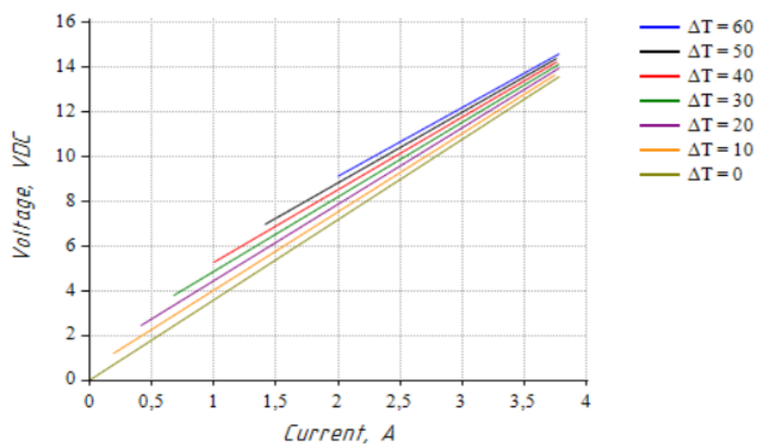
Voltage vs. Current (at T_{hot} = 27^{\circ}C )
