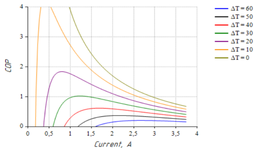
COP vs. Current (at T_{hot} = 50^{\circ}C )
