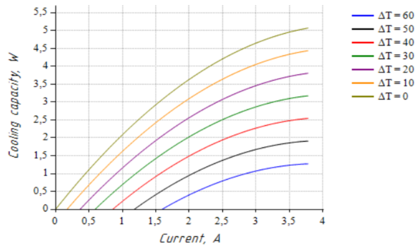
Cooling capacity vs. Current (at T_{hot} = 50^{\circ}C )
