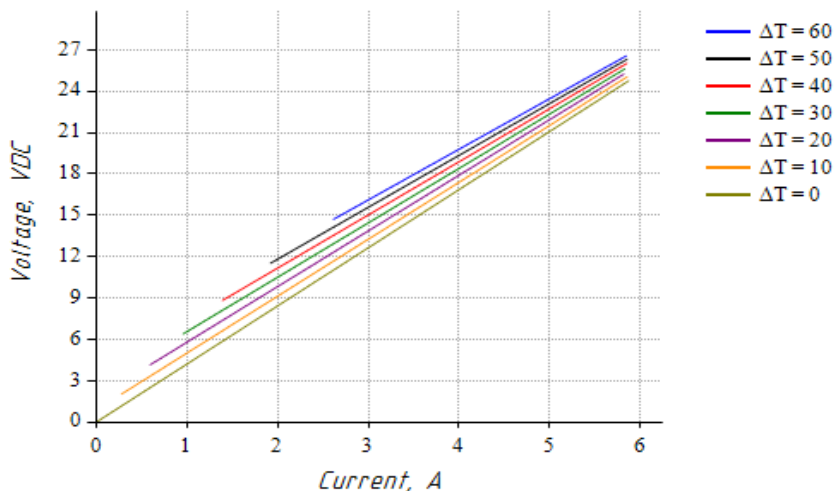
Voltage vs. Current (at T_{hot} = 50^{\circ}C )
