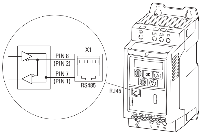
Figure 58: RJ 45 interface
