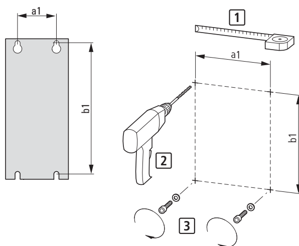
Figure 27: Mounting dimensions
