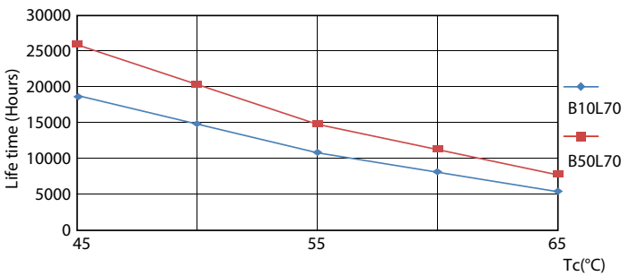
LEDtube 15K 4565 LifetimeVsTc-LED
