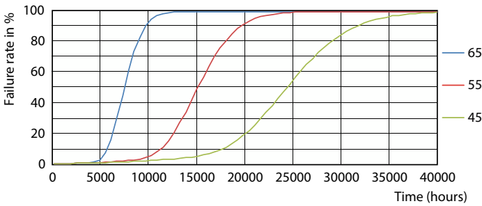
LEDtube 15K 4565 FailureRate-LED
