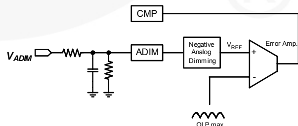
Figure 37. Analog Circuit Implementation
