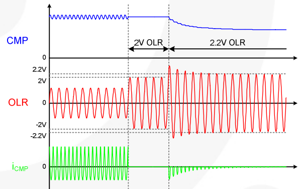
Figure 50. 2.2V Open-Lamp Regulation
