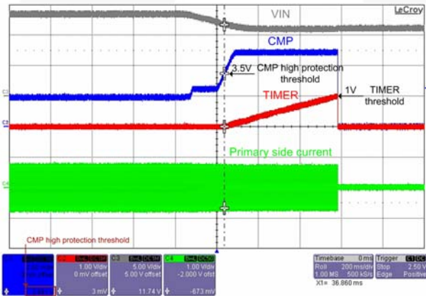
Figure 62. CMP-High Protection
