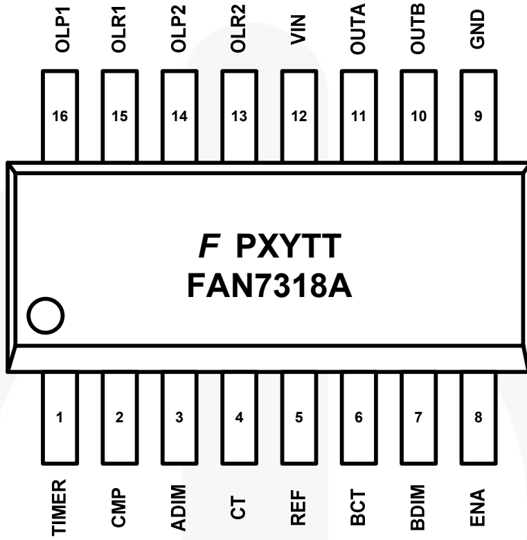
Figure 2. Package Diagram
