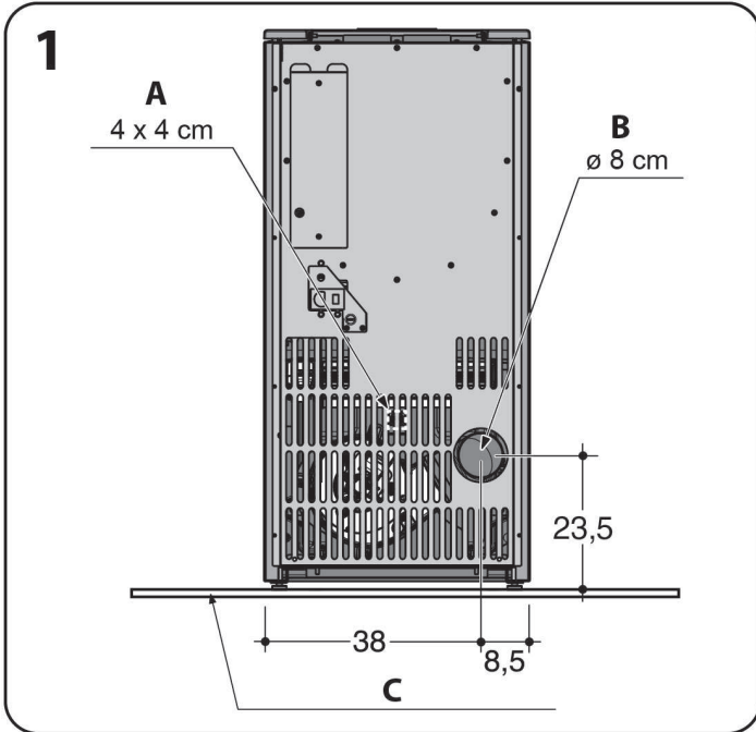
A. Combustion air inlet B. Smoke outlet C. Optional non-flammable floor protector
