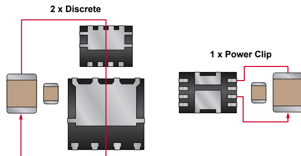
High Frequency Switching Loop Size Reduction
