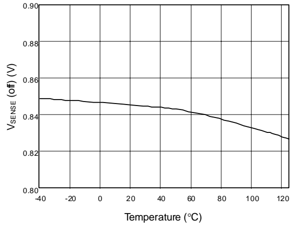
Fig. 2 V SENSE (off) vs. Temperature
