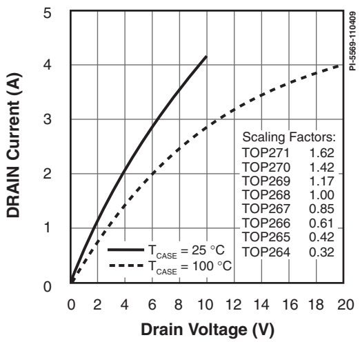
Figure 48. Output Characteristics.
