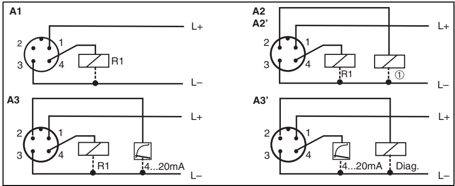
Fig. 3: Ceraphant T with M12x1 connector
