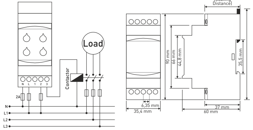
Connection Diagram & Dimensions for GKM-11
