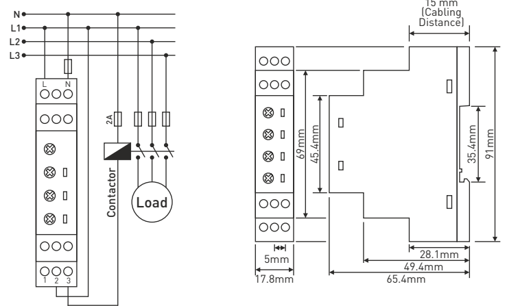
Connection Diagram & Dimensions for GKM-01
