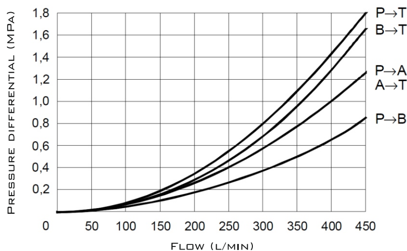
\Delta P -Q CHARACTERISTIC CURVES - SPOOL TYPE S, F, H, J, L, M, Q, U, V, W, C, D, K, Z
