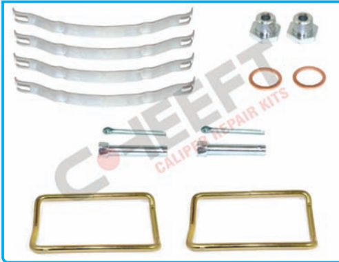
2248 - DX.195 Caliper Pad Retainer Repair Kit
