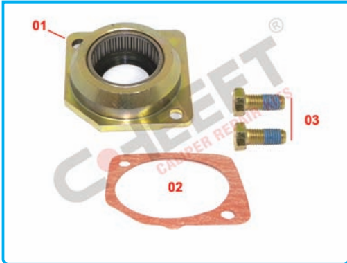
2236 - DX.195 Caliper Shaft Bearing
