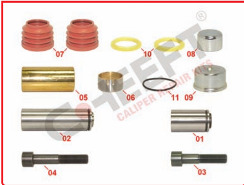
1184 - SB6/SB7 Caliper Guide & Seals Repair Kit
