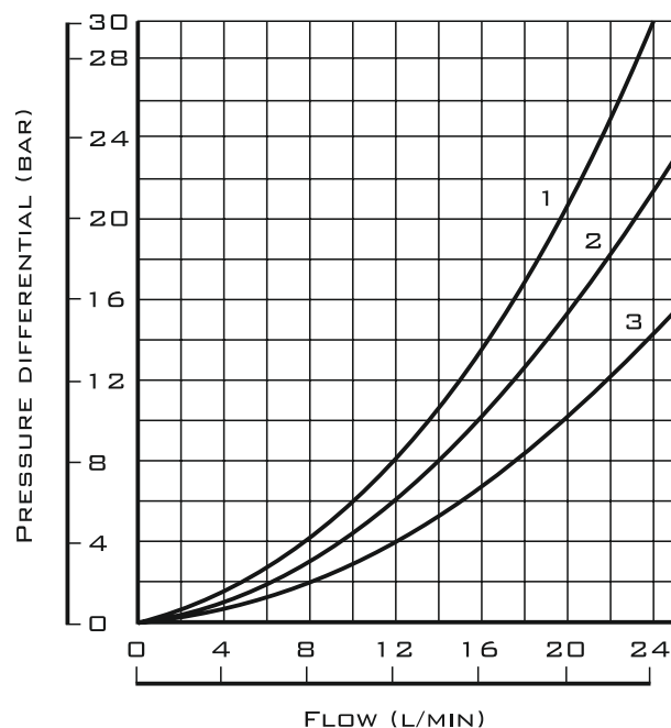
\Delta P -Q CHARACTERISTIC CURVES 4/2 DIRECTIONAL SEAT VALVE
