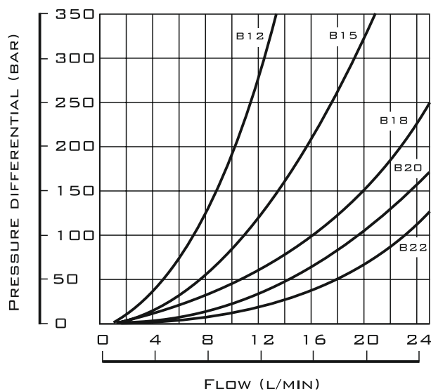
\Delta P -Q CHARACTERISTIC CURVES THROTTLE INSERT
