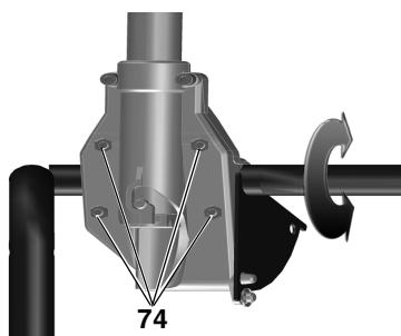
Setting guide bushings on rear leg mount:
