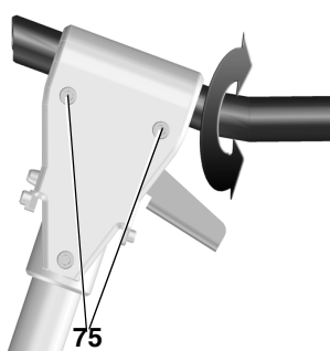
Tighten all Allen screws diagonally and evenly.
