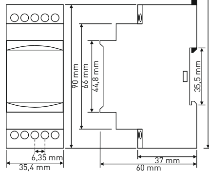
FK-14/14P Dimensions
