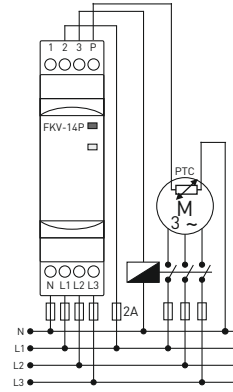
FKV-14/14P Connection Diagram
