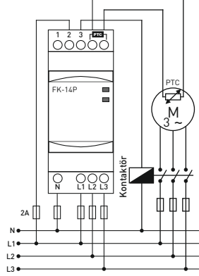
FK-14/14P Connection Diagram
