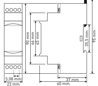
FKV-14/14P, FKV-03 Dimensions
