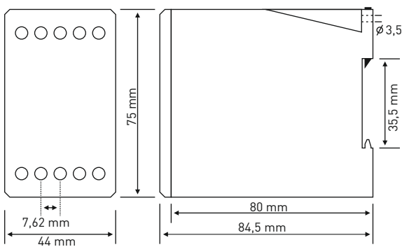
FK-04/04P, FS-R Dimensions
