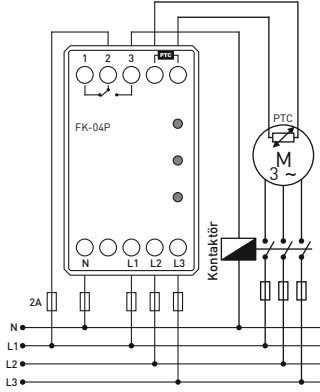
FK-04/04P Connection Diagram
