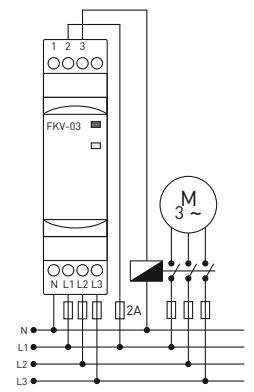
FKV-03 Connection Diagram
