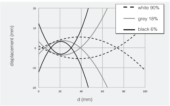
FQI7/B*-** spot dimension
