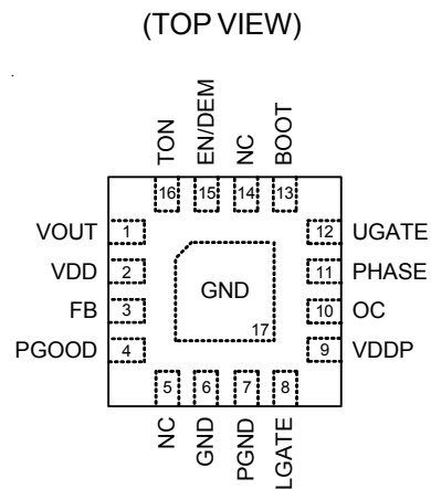
WQFN-16L 4x4 (RT8202L) WQFN-16L 3x3 (RT8202M)
