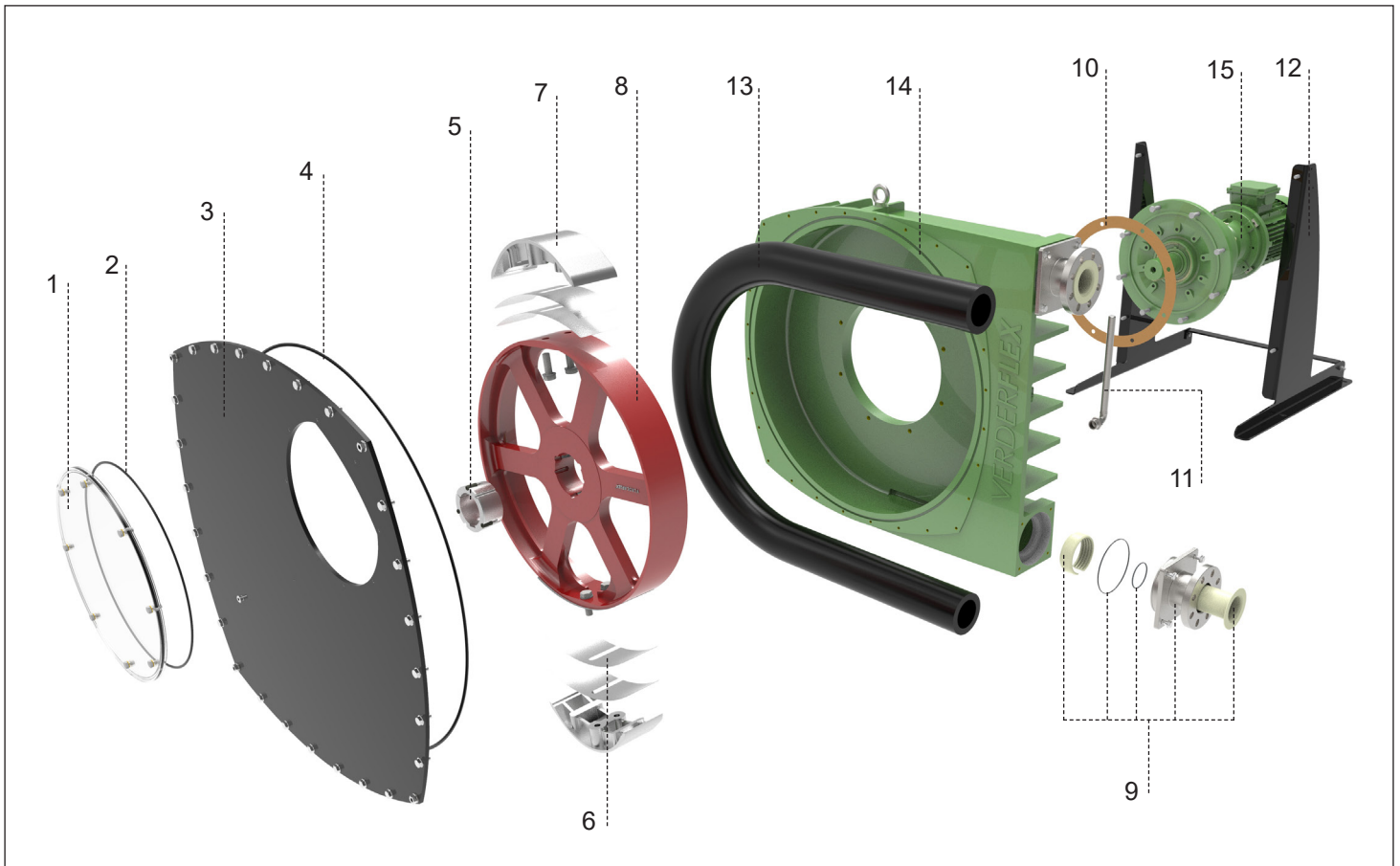
Figure 1 Layout VF 65-80 (Generic View)
