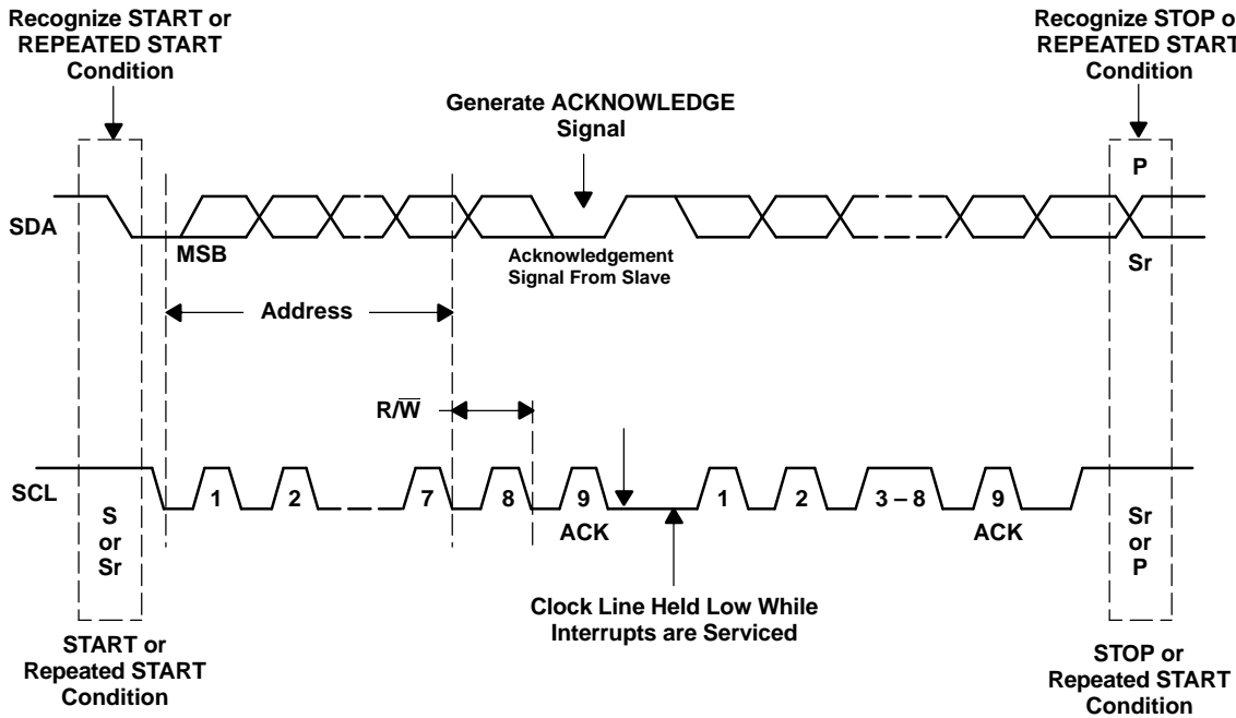
Figure 43. Bus Protocol
