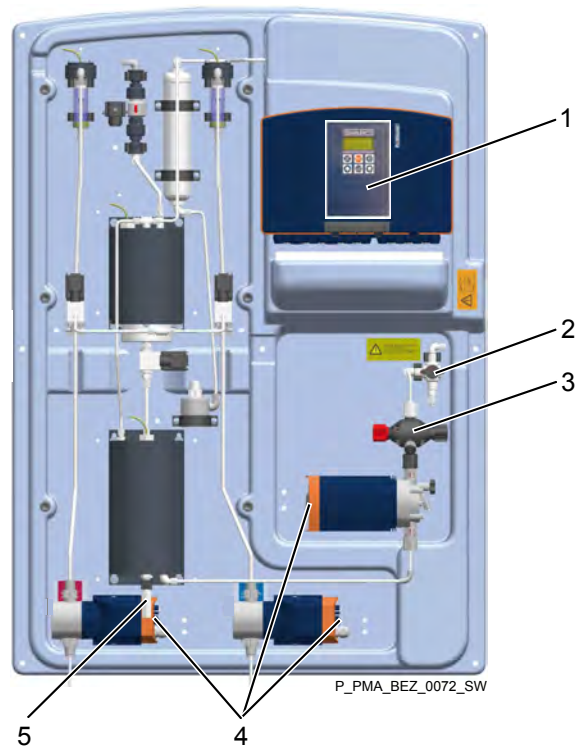
Fig. 13: Fully equipped CDLb 6
