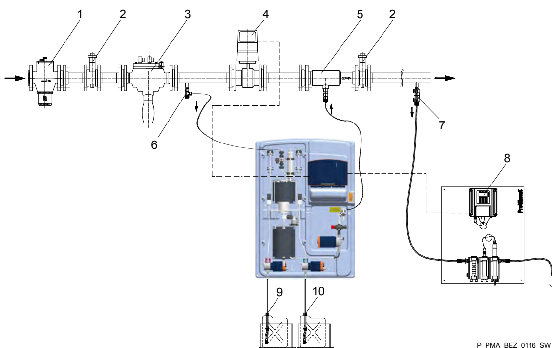
Fig. 8: Typical installation of a CDLb with internal pre-storage vessel
