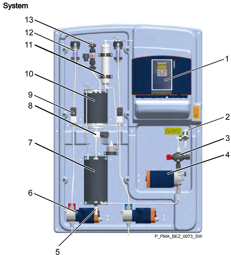
Fig. 5: System overview CDLb 22
