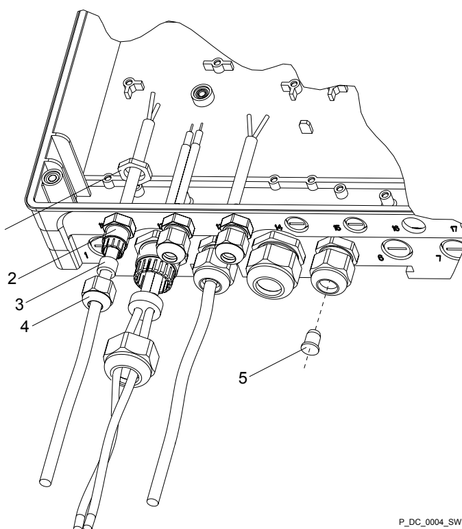
Fig. 11: Fitting the threaded cable gland
