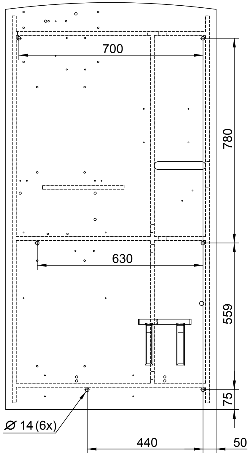
Drilling template for Bello Zon® CDLb 55 (Dimensions in mm)
