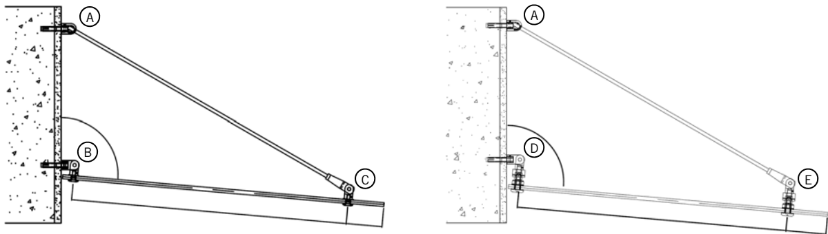
SINGLE & DOUBLE CANOPY END VIEW SECTION
