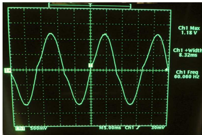
No Load Open Circuit Screen shot
