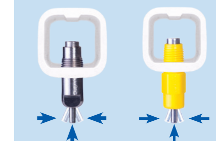
LUBING TOP-Nipple Art. 4022 (left) and the TOP-Combinipple Art. 4024-00 (right) with sideways action for rearing.
