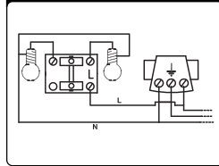
Connection Diagram
