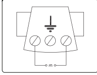
Connection Diagram
