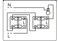
Connection Diagram
