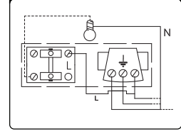
Connection Diagram
