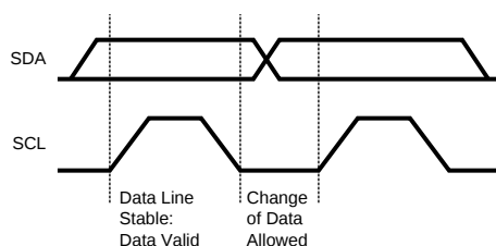
Figure 20. Bit Transfer
