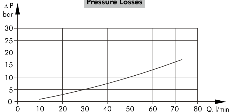
Pressure Losses
