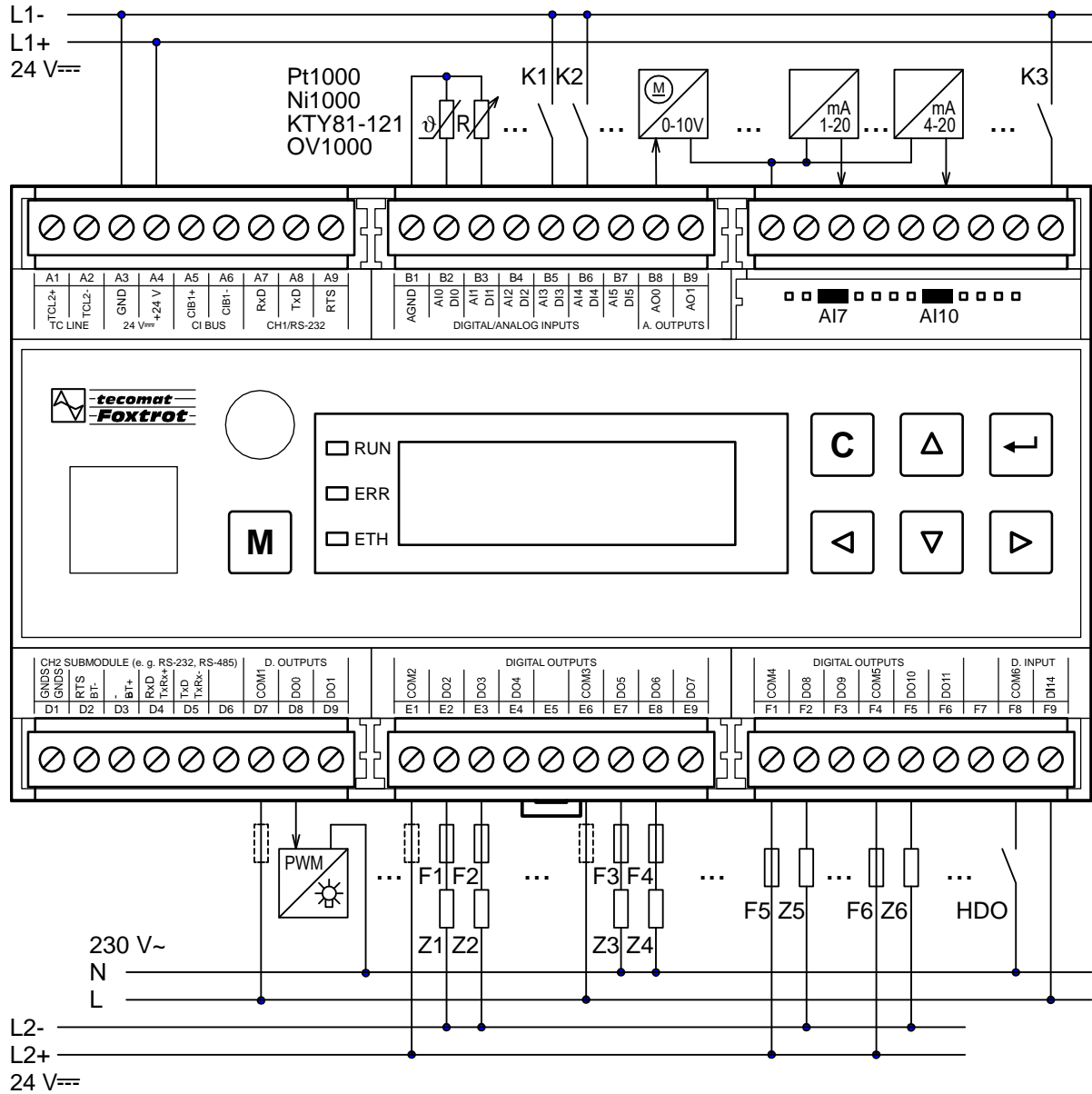
Fig. 4.1 Example of connection of binary and analog inputs/outputs of basic module CP-1016
