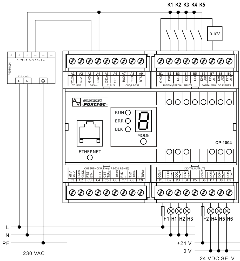
Fig. 4.1 Elementary connection of CP-1004 module
