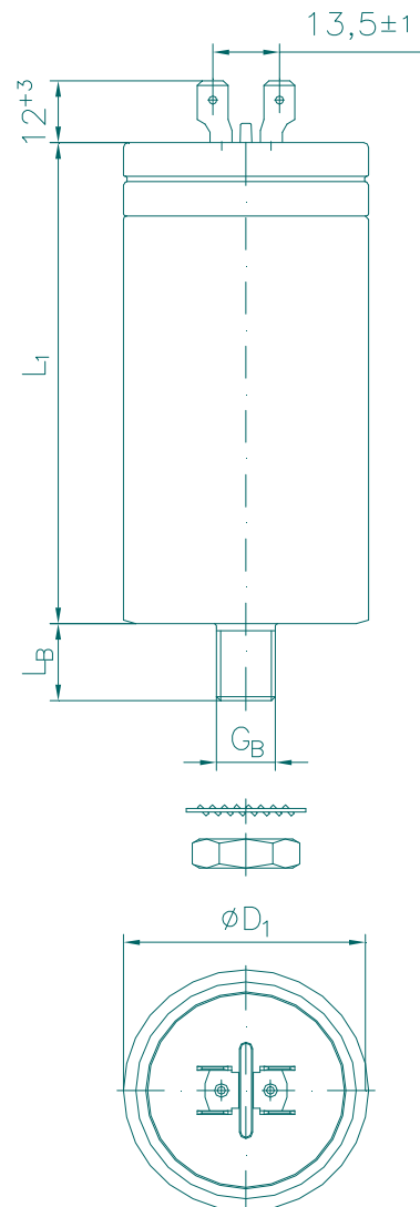
outline drawing
