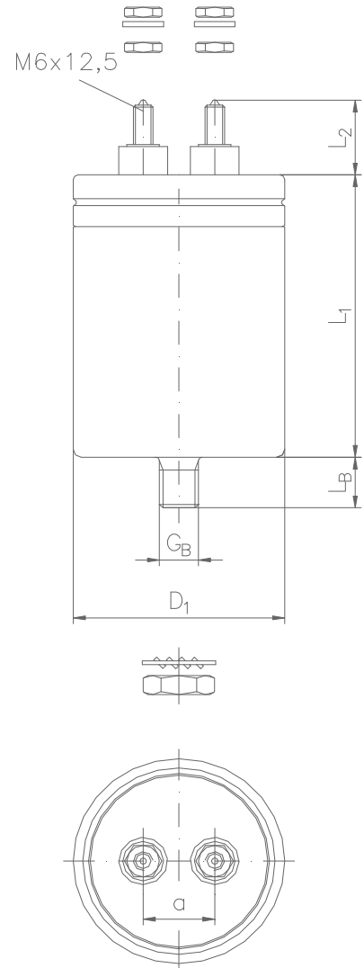
outline drawing
