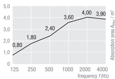
TOPIQ® Sonic element, rectangular 1800 x 1200 mm, Assembly height 300 mm
