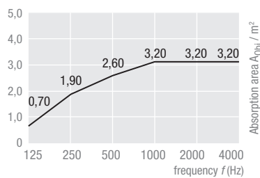
TOPIQ® Sonic element, rectangular 1800 x 1200 mm, Assembly height 150 mm
