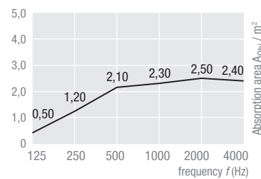
TOPIQ® Sonic element, square 1200 x 1200 mm, Assembly height 150 mm
