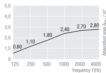
TOPIQ® Sonic element, square 1200 x 1200 mm, Assembly height 300 mm
