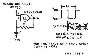
Fig. 18 - Astable multivibrator.
