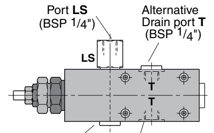
Alternative LS port Port T (BSP 1/4"); Must be connected directly to tank!
