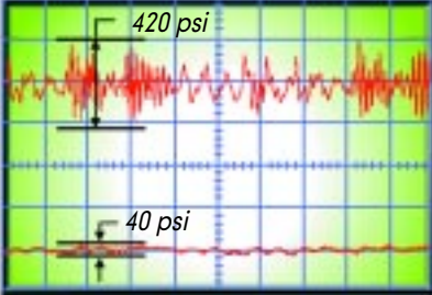
The Suppressor reduces pulsations from a piston pump at 2000 psi at 1800 rpm from 420 psi to 40 psi.
