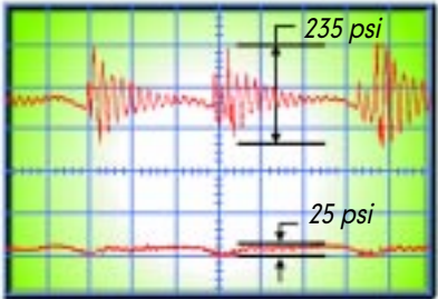
The Suppressor reduces pulsations from a piston pump at 4000 psi at 1800 rpm from 235 psi to 25 psi.
