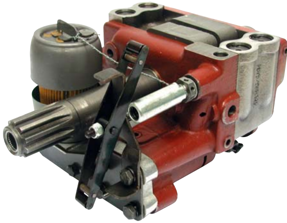
Hydraulic pump - earlier model MF0618
