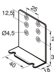
Fig. 7: Part No. 803 799
