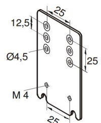
Fig. 9: Part No. 803 800
