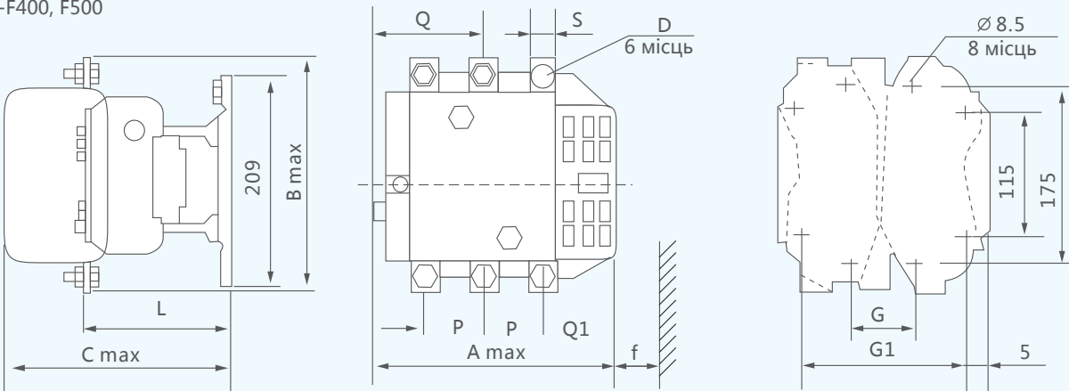
CJX2-F400, F500
