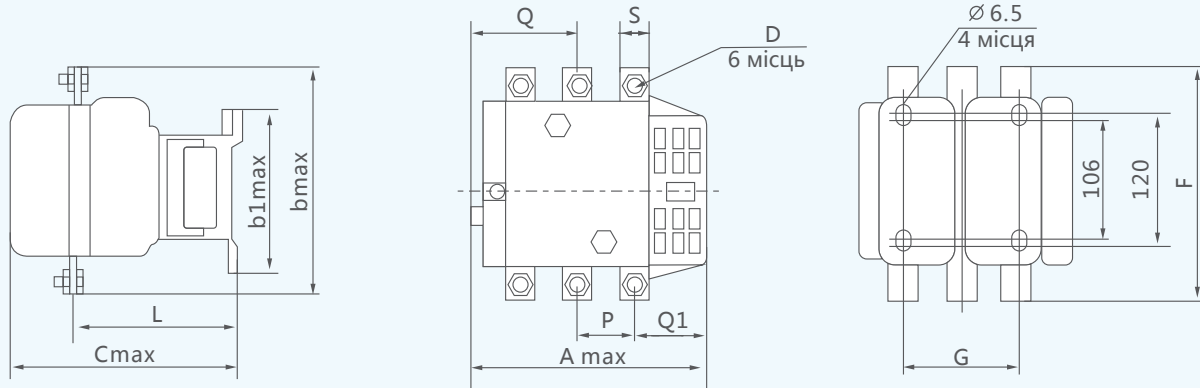
CJX2-F115-F330
