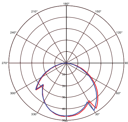
CO Plane beam angle(50%): 119.9(DEG) C90 Plane beam angle(50%): 118.8(DEG)
